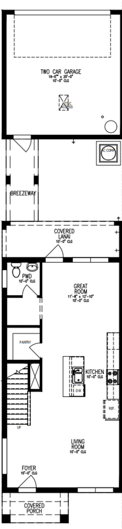
HARBOR 1ST FLOOR PLAN
