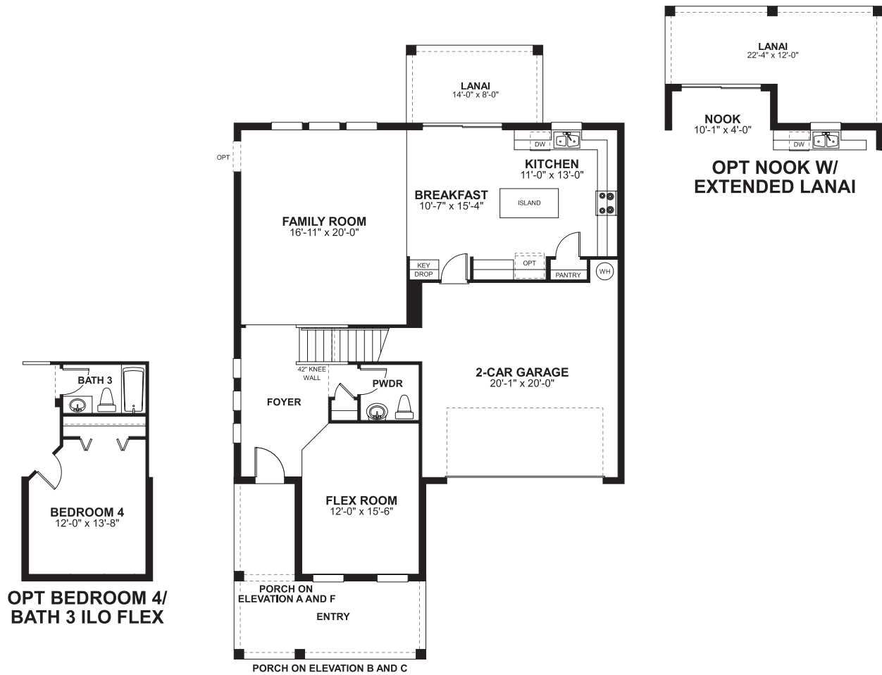
FIRST FLOOR
